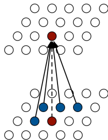
PixelCNN
